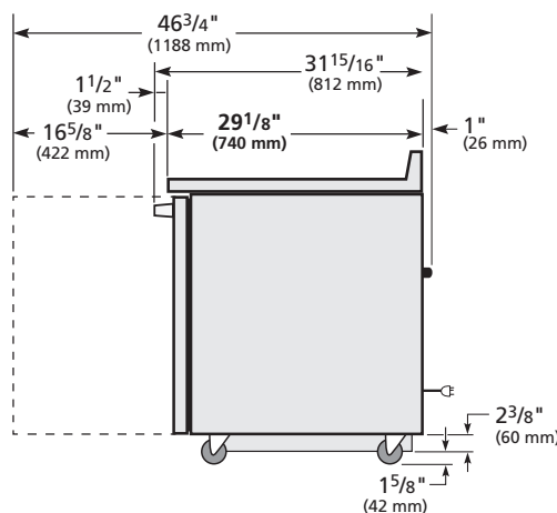
RIGHT VIEW
